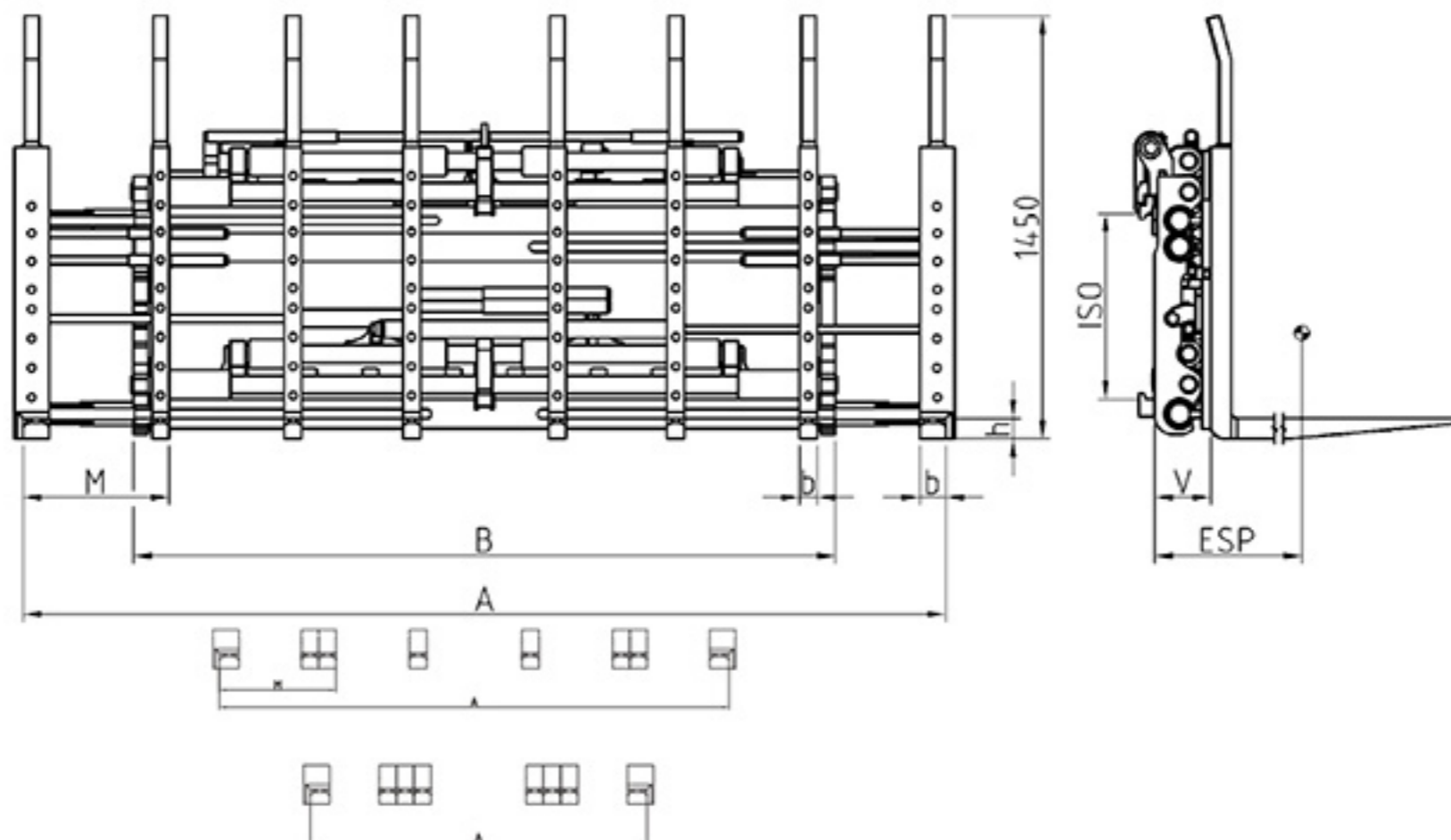
type VPK for 2-3-4 pallets
